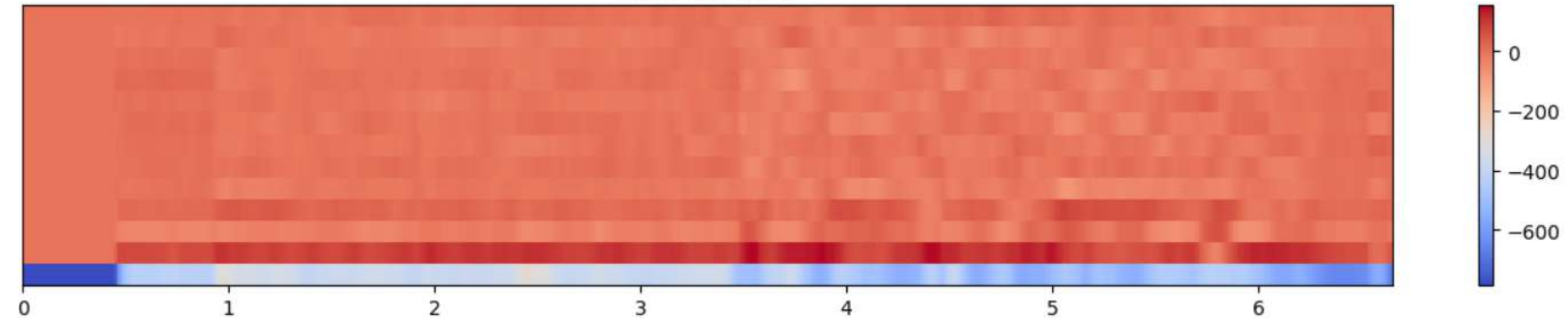
MFCC Features
