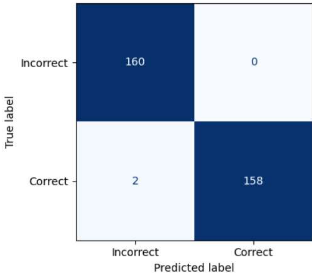
Confusion Matrix
